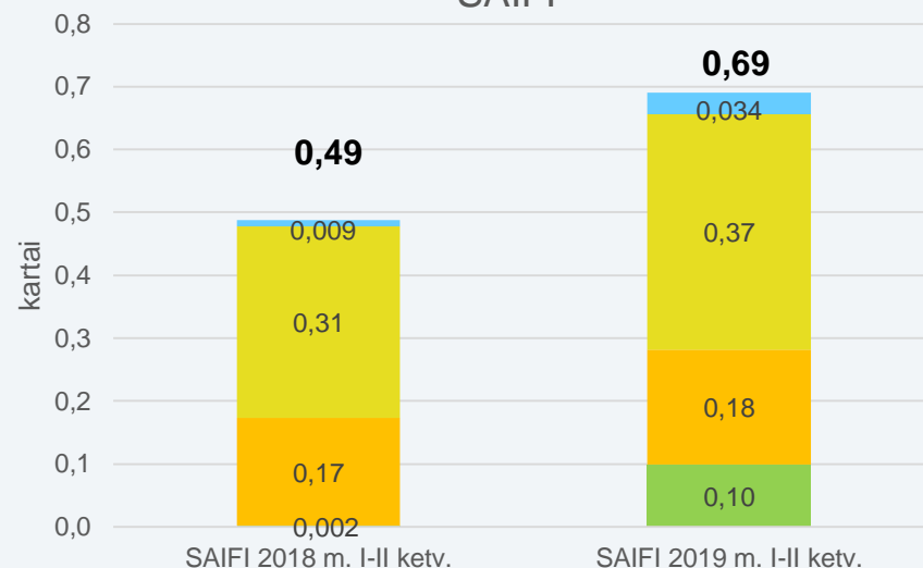
SAIFI
