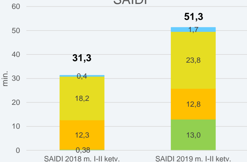
SAIDI
